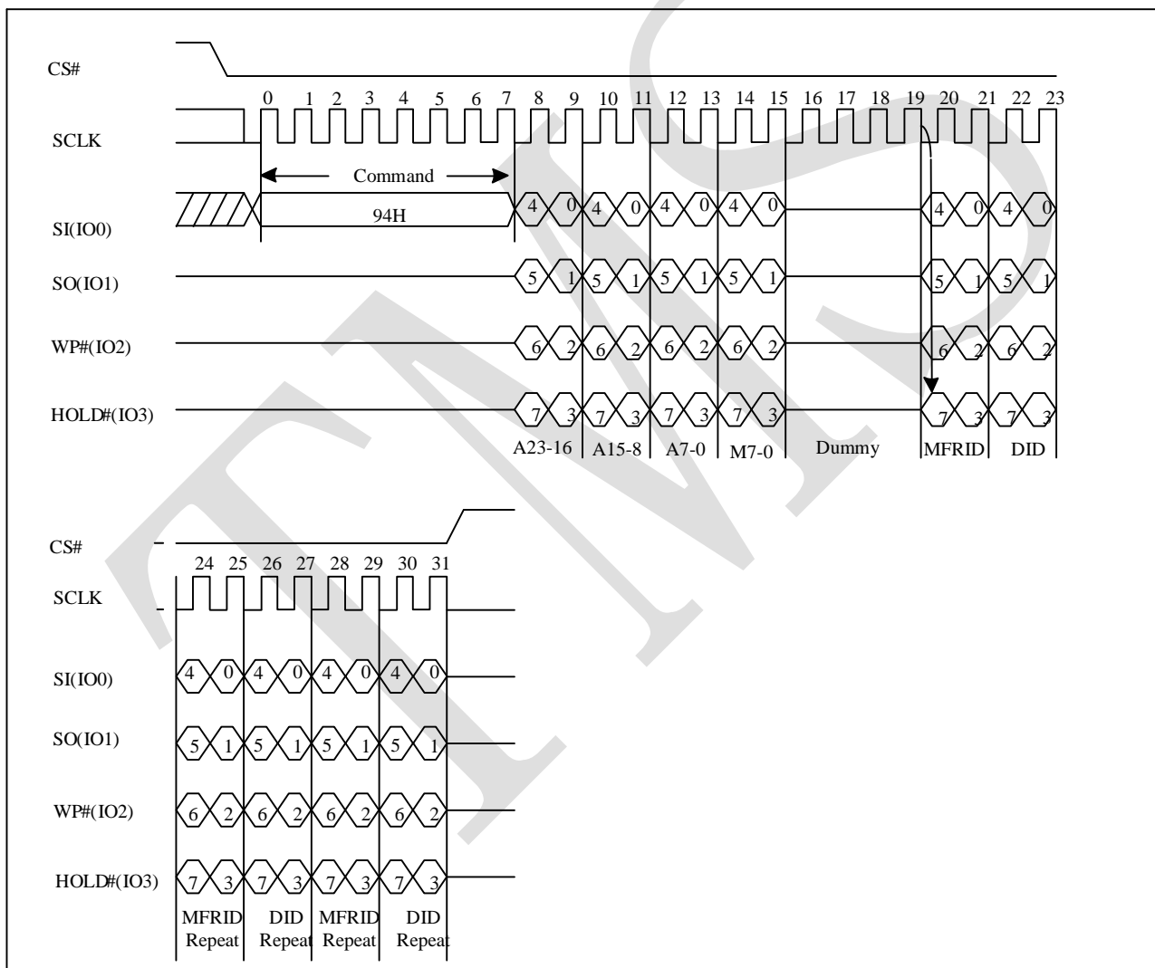
Figure 5-33 QUAD I/O Read Electronic Manufacturer & Device ID (QREMS) Sequence (Command 94)
