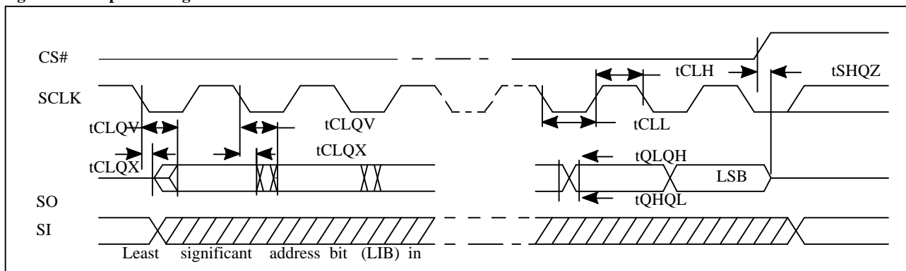
Figure 4-5 Output Timing
