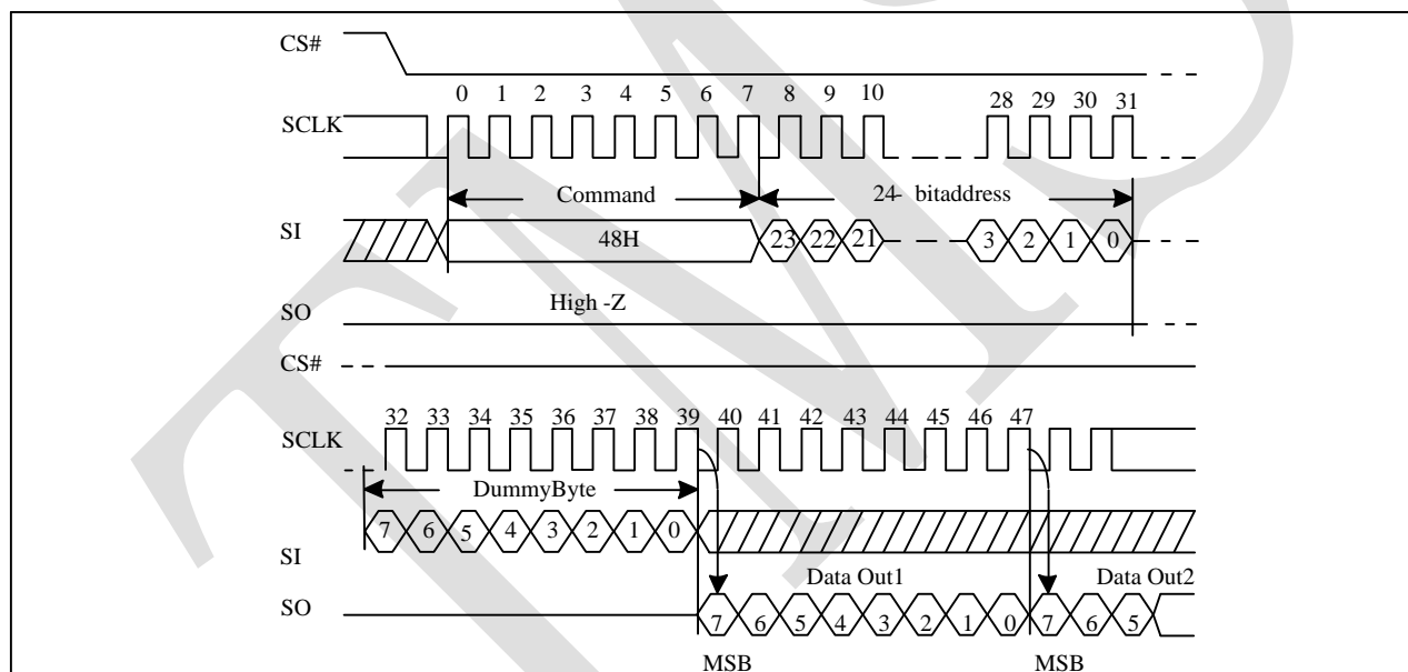
Figure 5-27 Read Security Registers (RDSCUR) Sequence (Command 48)
