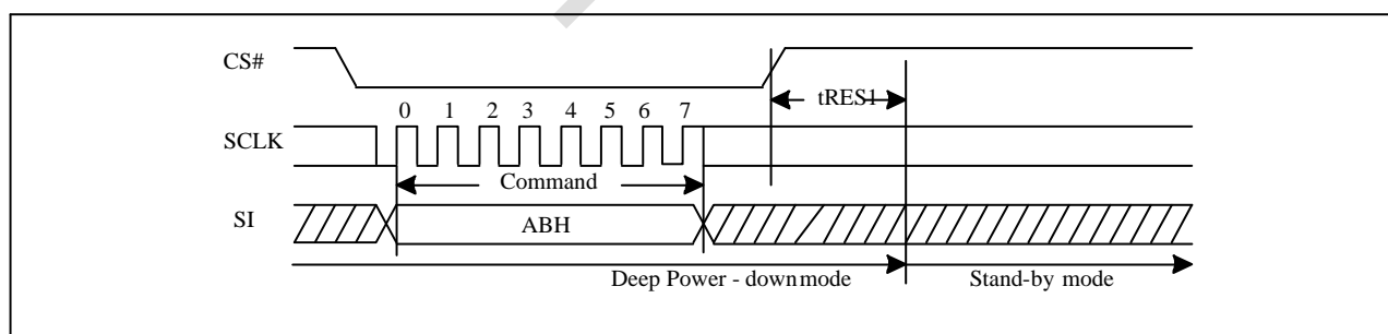
Figure 5-30 Release from Deep Power-down (RDP) Sequence (Command AB)
