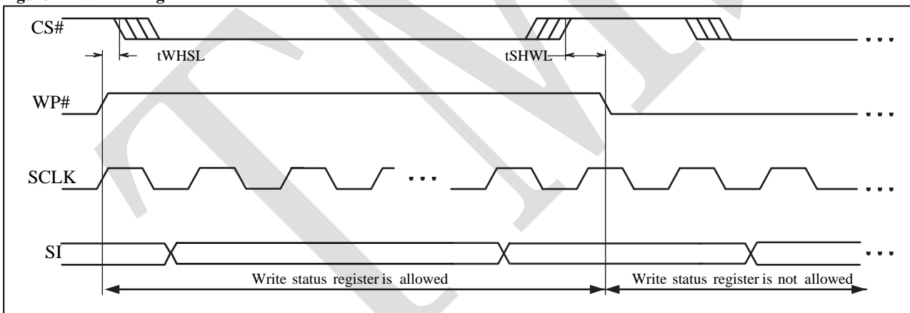
Figure 4-7 WP Timing
