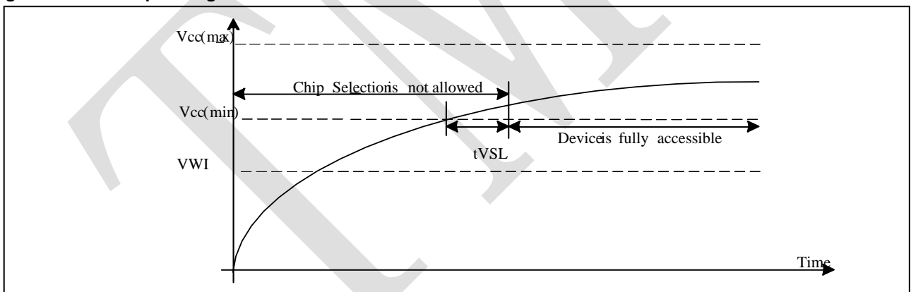
Figure 4-9 Power-Up Timing
