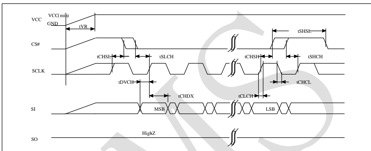
Figure 4-7 AC Timing at Device Power-Up
