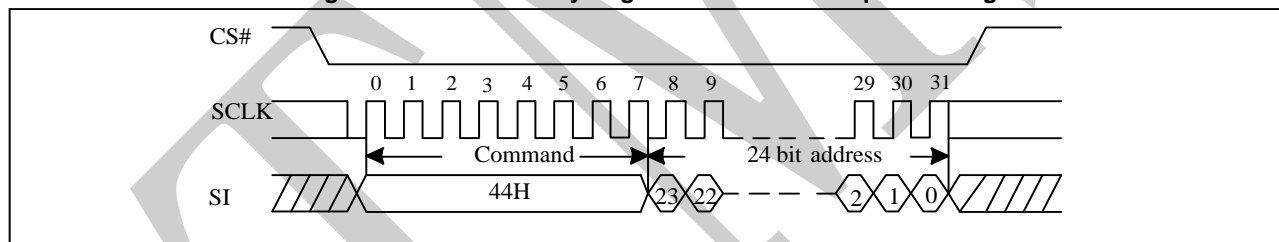
Figure36. Erase Security Registers command Sequence Diagram
