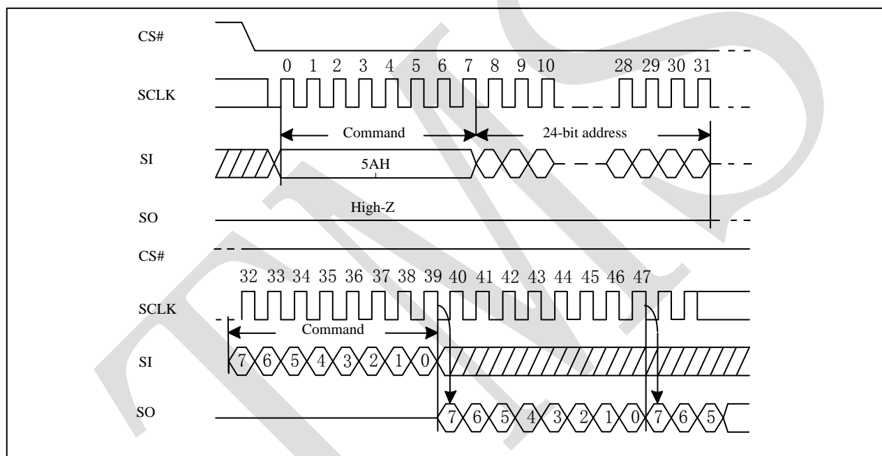
Figure 5-43 Read Serial Flash Discoverable Parameter(RDSFDP) Sequence
