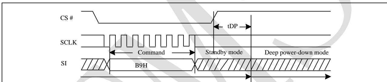
Figure 5-28 Deep Power-down (DP) Sequence (Command B9)
