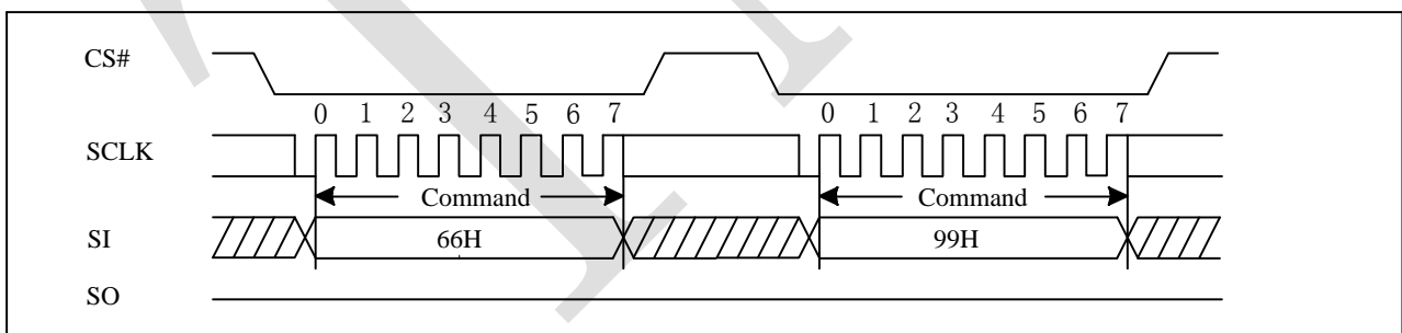
Figure 5-39 Reset Sequence
