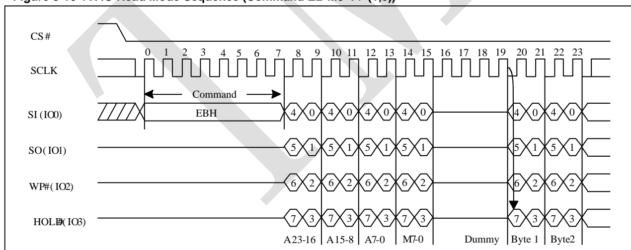
Figure 5-16 4 X IO Read Mode Sequence (Command EB M5-4 ≠ (1,0))
