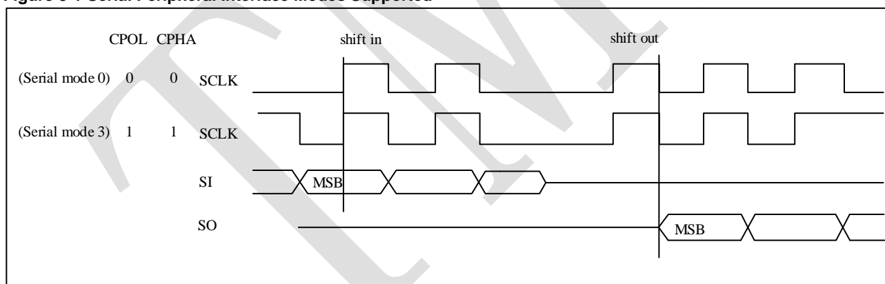
Figure 3-1 Serial Peripheral Interface Modes Supported
